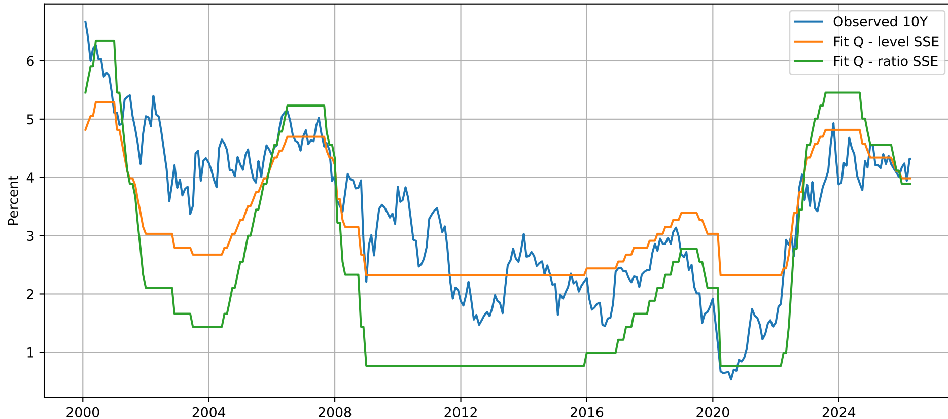
Observed vs model-implied 10Y yield under Q
